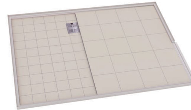
Water stop line design to guarantee 100% leakproof
