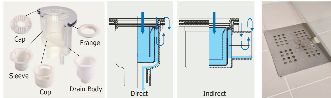
Removable design, easy clean Deodorant design
